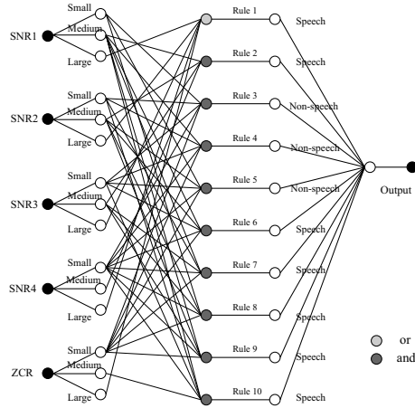
Fig. 3. Rule base
