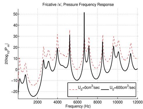
Figure 1: Frequency response for non-zero mean volume velocities. The area function used corresponds to the fricative /x/. The spectrum for U_0 = 600 \text{ cm}^3/\text{sec} has been downshifted by 10dB for better visualization. Effects at the lower frequencies may be observed, i.e. the relative magnitude of the first two peaks has changed.
