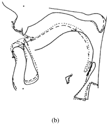
Figure 2: 2a: Mid-sagittal profiles of the vocal tract for vowel [a]. For each profile, the phonetic score, the position of the main constriction (Constric) w.r.t. the glottis and the constriction area in \text{cm}^2 are given. 2b: X-ray mid-sagittal profiles for [a]: [aba] (solid line), [maf] (dashed line), [vwal] (dotted line)
