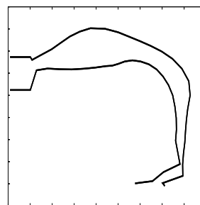
Score = 0.2 Constrict = 2.3 Area = 0.2
