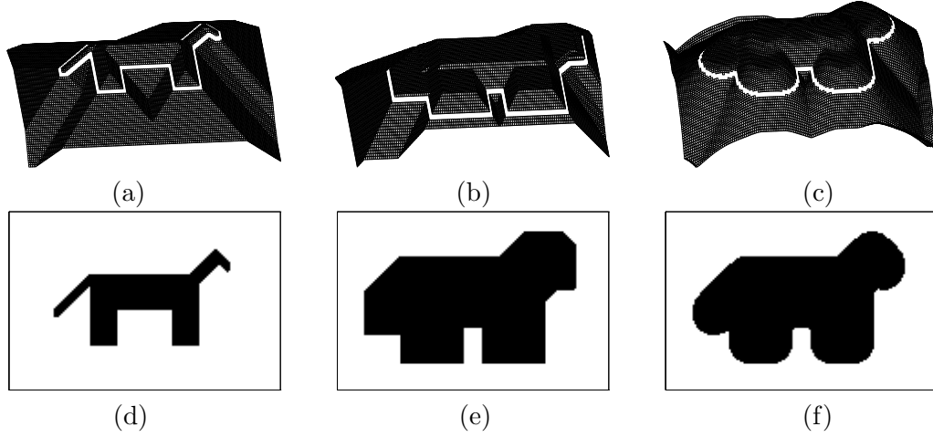
Figure 5: (a) Original digital gray-level image f and its contour at level=0. (b) Flat dilation f \oplus B of f by a discrete disk, i.e. a square of (2t+1) \times (2t+1) pixels with t = 5 . (c) Dilation of f by a Euclidean disk at scale t = 5 by running the PDE \partial\delta/\partial t = \|\nabla\delta\|_2 for t \in [0, 5] with initial condition \delta(x, y, 0) = f(x, y) . (d) Binary image S from thresholding f at level=0. (e) Binary image S \oplus B from thresholding f \oplus B at level=0. (f) Binary image from thresholding the evolving image surface in (c) at level=0.
